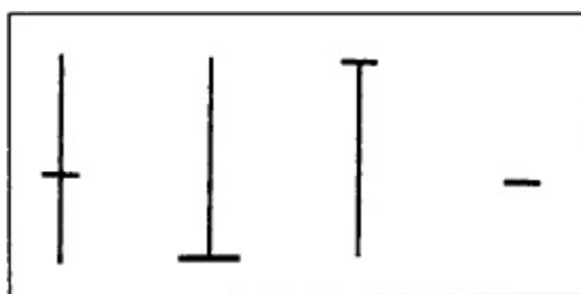
Figure 12.5 Doji candlesticks.
