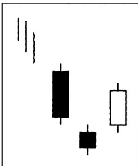
Figure 12.9 Morning star +.
