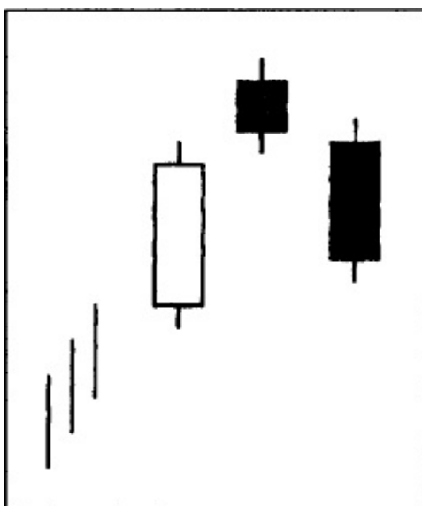
Figure 12.8 Evening star -.
