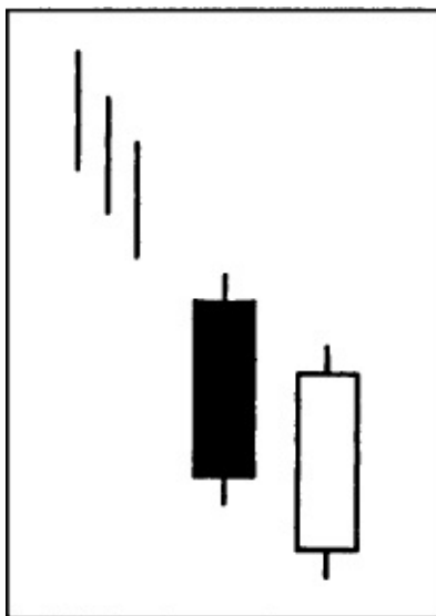
Figure 12.7 Piercing line +.
